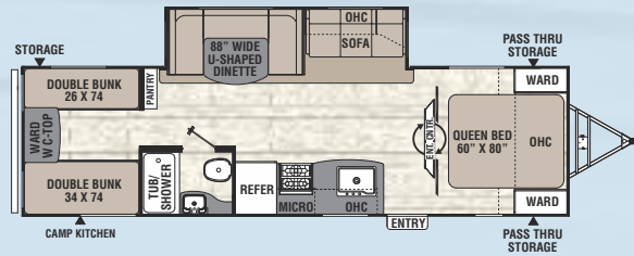
292 BHSLE / Exterior Length 33' 5"
