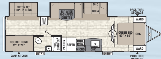
310 BHSLE / Exterior Length 35' 7"
