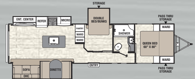
323 BHDSLE / Exterior Length 36' 11"
