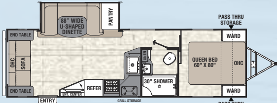
279 RLDSE / Exterior Length 31' 11"
