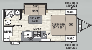
192 RBS / Exterior Length 22' 6"
