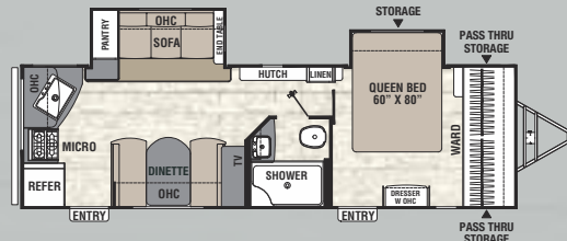
276 RKDS / Exterior Length 31' 6"
