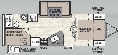
257 BHS / Exterior Length 28' 7"
