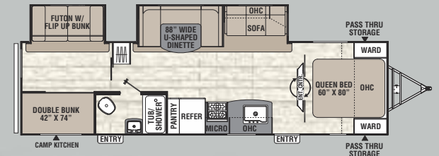
310 BHDS / Exterior Length 35' 7"
