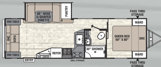
279 RLDS / Exterior Length 31' 11"
