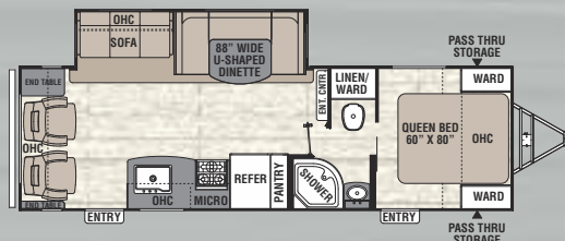
281 RLDS / Exterior Length 31' 8"
