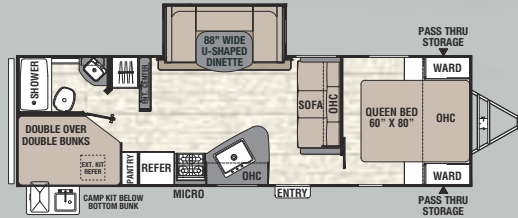
275 BHS / Exterior Length 31' 9"
